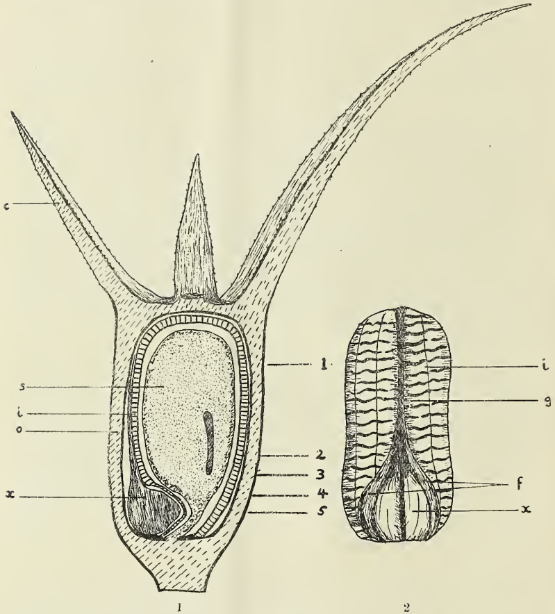
FIG. 1. Carpacoce spermacoccea . View of the fruit, with the outer layer of the ovary wall removed, facing the parenchymatous swelling \times 15 . i , wrinkled inner layer of the ovary wall; f , flap-like extension of inner layer; x , parenchymatous swelling; g , groove.
